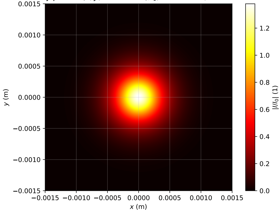
Intensity profile I(x, y, z = 0.796m)/I_0 , Pin=1.0Pcr, artificial time
